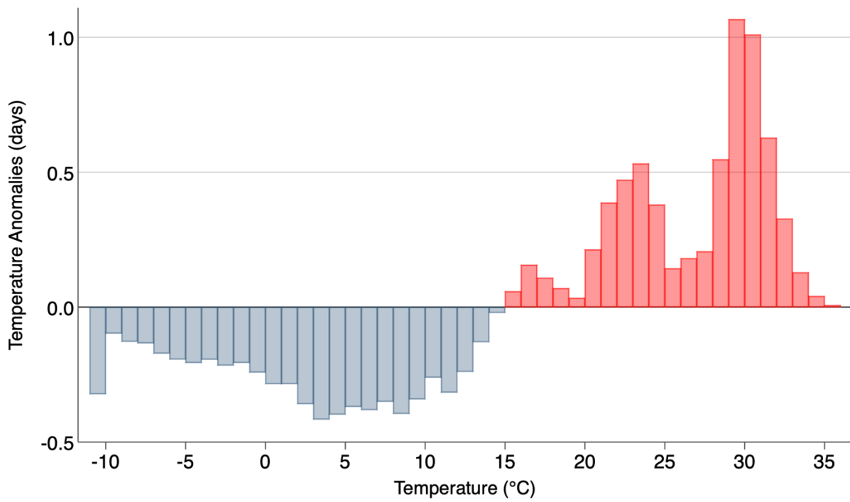
Figure 3. Mean values of temperature anomalies experienced by an average county in each 1°C interval in China from 2003 to 2020. Temperature anomalies are calculated by subtracting the average temperature bin over the average of the past ten years.
