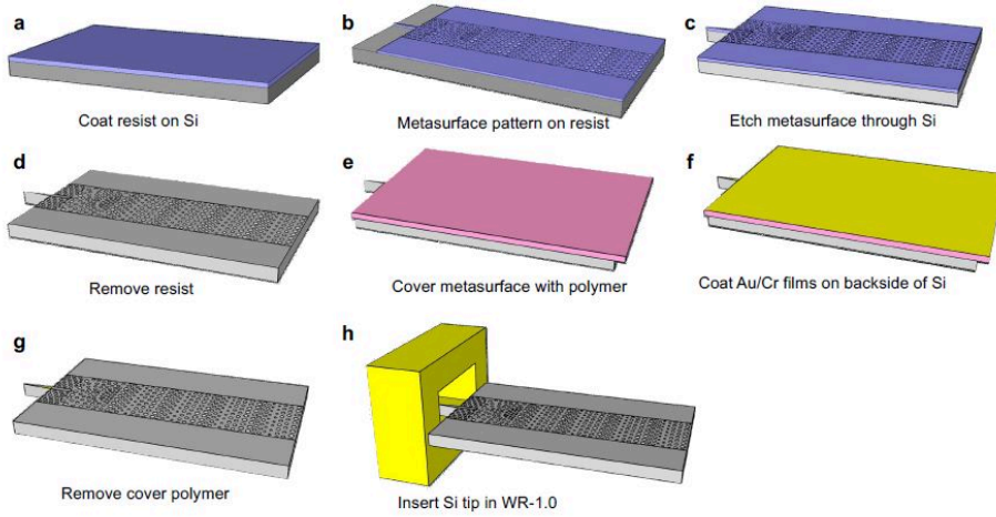
Figure 2. Fabrication technology for waveguide-integrated superheterodyne THz antenna
