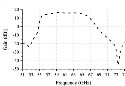
Realized gain of the filtering FPC antenna.
