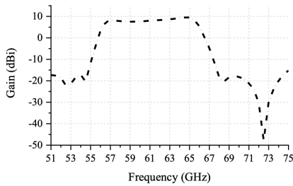
Realized gain of the filtering antenna source.
