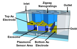
Fig. 2. Schematic of Microfluidic Biosensing Chip.
